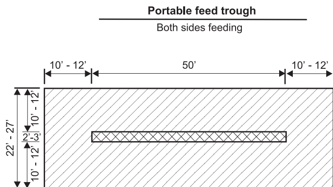
Figure 4. Geotextile pad for feeding with portable trough.
